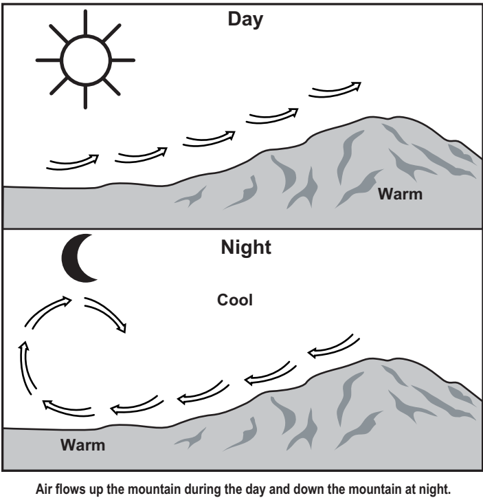
Figure 1-1. Anabatic and Katabatic Winds.
